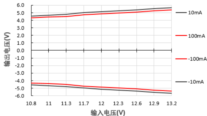
输出电压Vs输入电压@A1205S-1WR3
