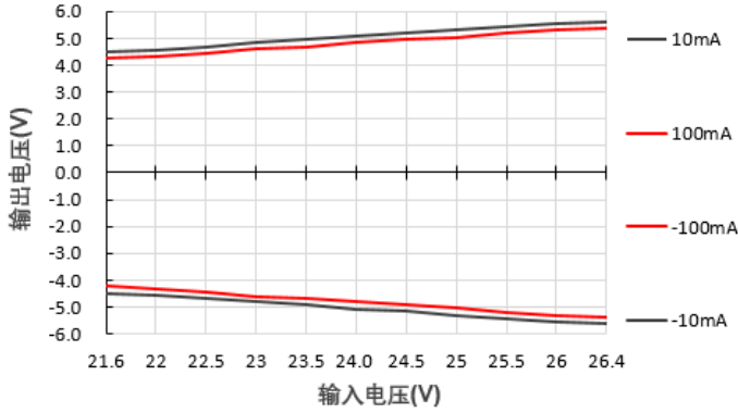
输出电压Vs输入电压@A2405S-1WR3
