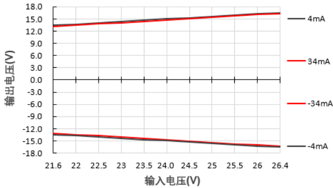
输出电压Vs输入电压@A2415S-1WR3
