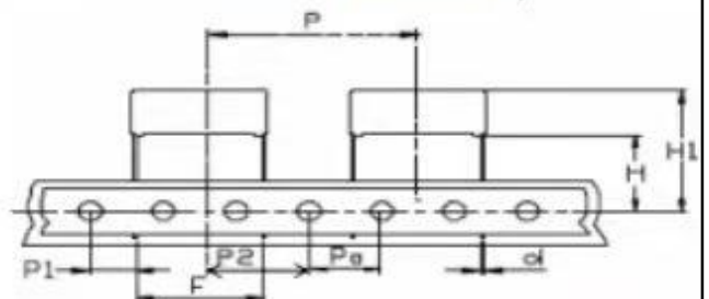
Fig 4 Pitch: 22.5/27.5 Po=12.7
