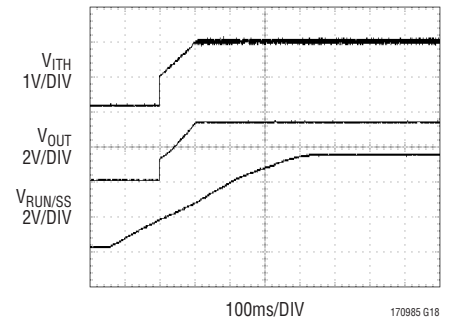
Soft-Start Up
