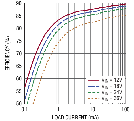
Burst Mode Efficiency, V_{OUT} = 24\text{V} , L = 15\mu\text{H}
