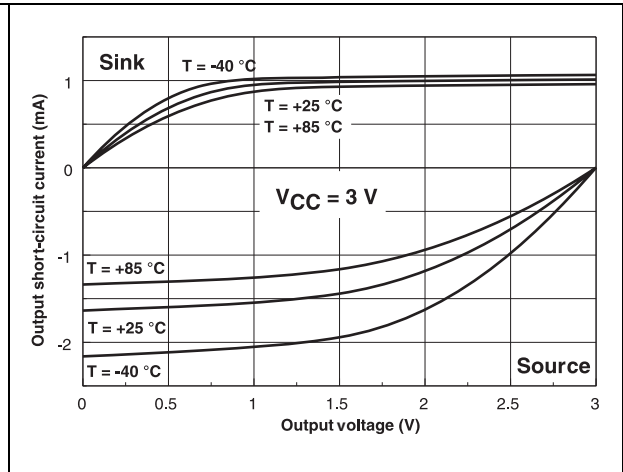
Figure 8. Output short-circuit current vs. output voltage at V_{CC+} = 3 V
