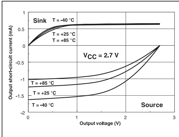
Figure 7. Output short-circuit current vs. output voltage at V_{CC+} = 2.7 V
