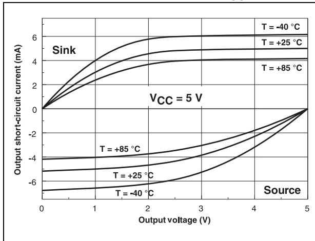
Figure 9. Output short-circuit current vs. output voltage at V_{CC+} = 5 V
