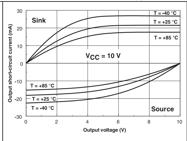
Figure 10. Output short-circuit current vs. output voltage at V_{CC+} = 10 V
