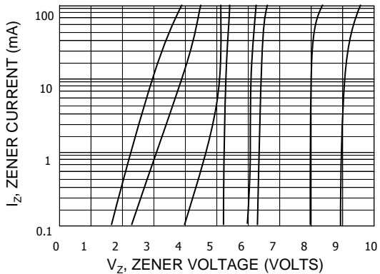
FIG. 7 - ZENER VOLTAGE VS. ZENER CURRENT V Z = 3.3 thru 10 VOLTS
