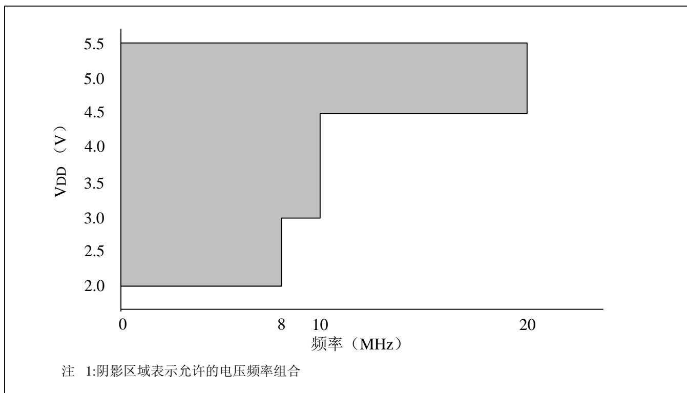
图 13-1-1: MDT10F684 电压-频率图, -40^{\circ}\text{C} \leq \text{TA} \leq +85^{\circ}\text{C}
