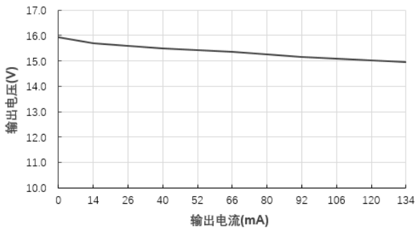
输出电压Vs输出电流(Vin=12V)@F1215S-2WR2
