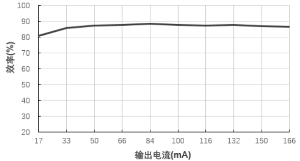
效率Vs输出电流(Vin=5V)@F0512S-2WR2
