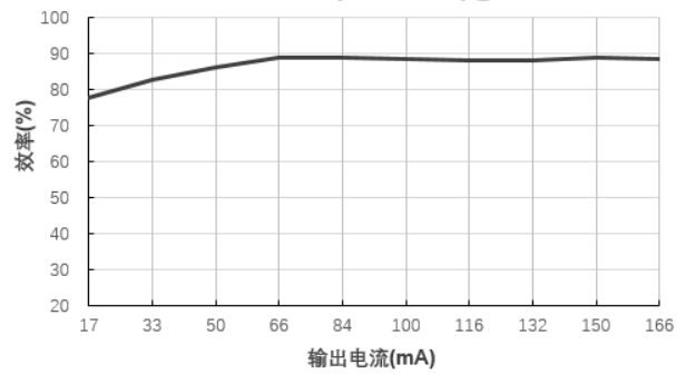
效率Vs输出电流(Vin=24V)@F2412S-2WR2
