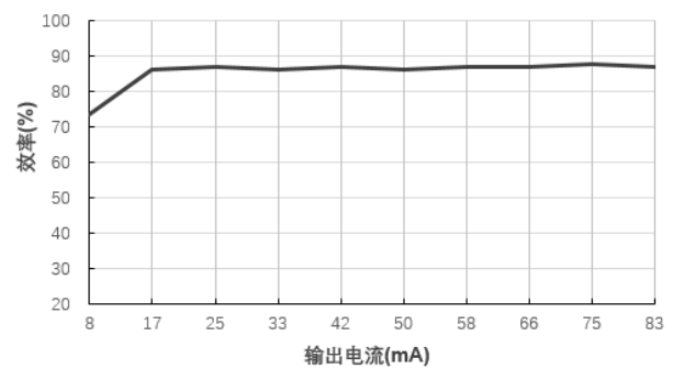
效率Vs输出电流(Vin=5V)@F0524S-2WR2
