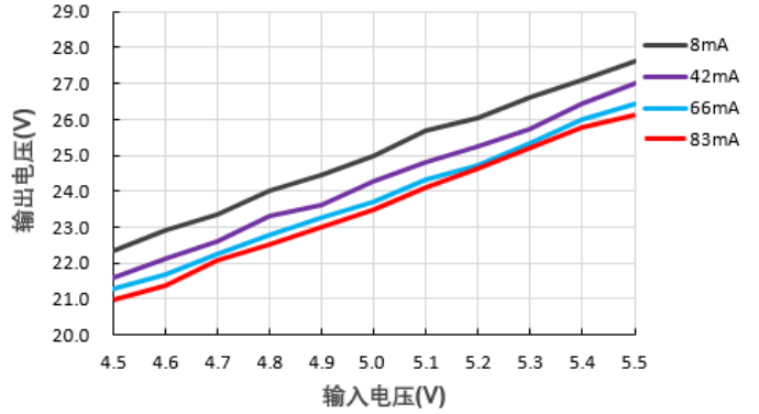
输出电压Vs输入电压@F0524S-2WR2
