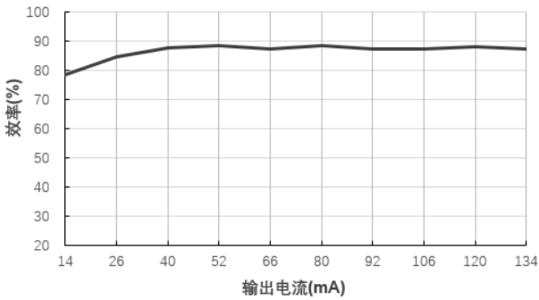
效率Vs输出电流(Vin=5V)@F0515S-2WR2
