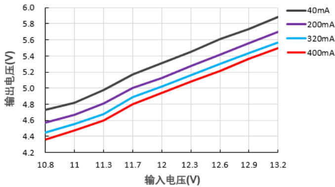
输出电压Vs输入电压@F1205S-2WR2
