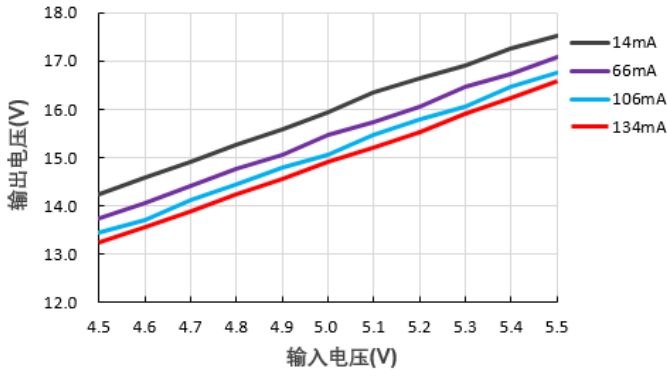
输出电压Vs输入电压@F0515S-2WR2
