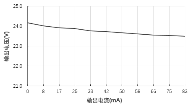
输出电压Vs输出电流(Vin=24V)@F2424S-2WR2
