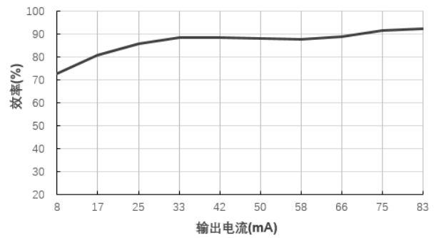
效率Vs输出电流(Vin=24V)@F2424S-2WR2
