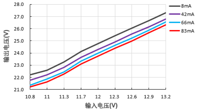
输出电压Vs输入电压@F1224S-2WR2
