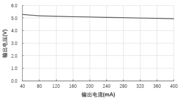
输出电压Vs输出电流(Vin=24V)@F2405S-2WR2
