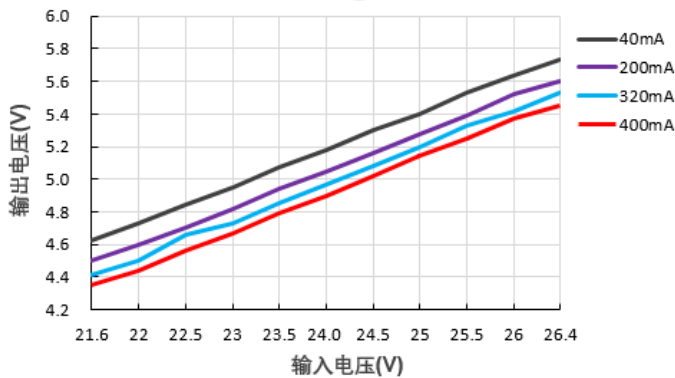
输出电压Vs输入电压@F2405S-2WR2
