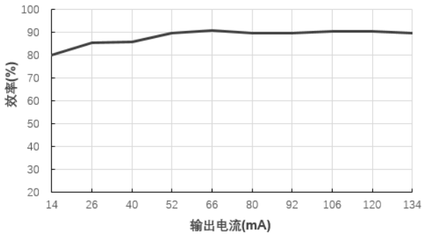
效率Vs输出电流(Vin=24V)@F2415S-2WR2
