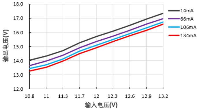
输出电压Vs输入电压@F1215S-2WR2
