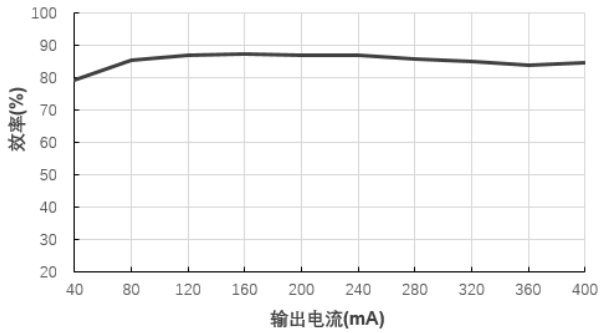
效率Vs输出电流(Vin=5V)@F0505S-2WR2
