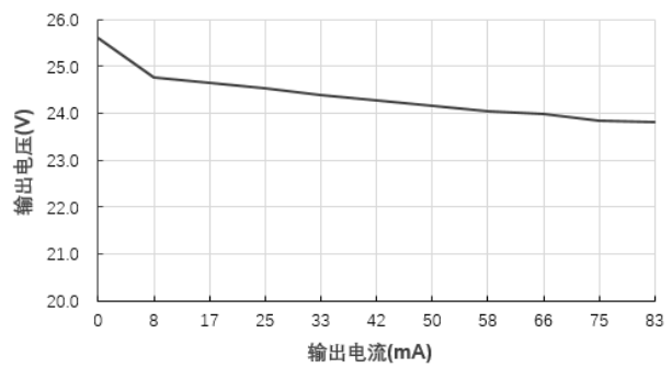
输出电压Vs输出电流(Vin=12V)@F1224S-2WR2
