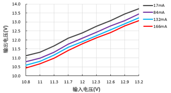
输出电压Vs输入电压@F1212S-2WR2
