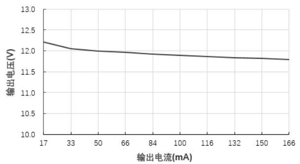
输出电压Vs输出电流(Vin=24V)@F2412S-2WR2
