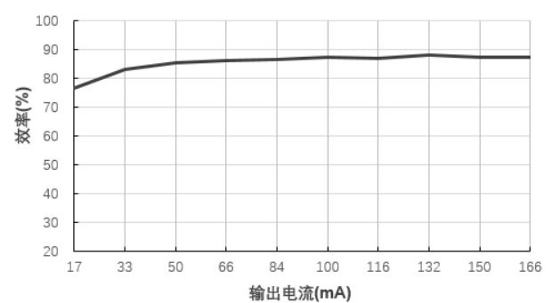
效率Vs输出电流(Vin=12V)@F1212S-2WR2
