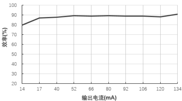
效率Vs输出电流(Vin=12V)@F1215S-2WR2
