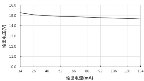
输出电压Vs输出电流(Vin=24V)@F2415S-2WR2
