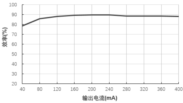
效率Vs输出电流(Vin=24V)@F2405S-2WR2
