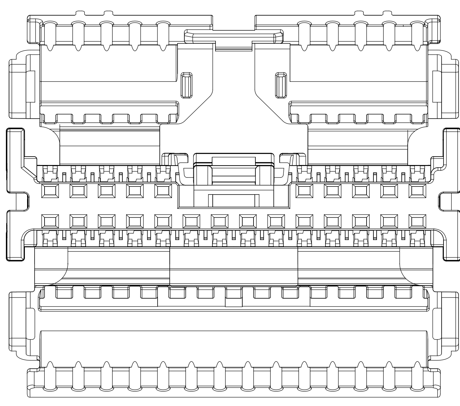
24 CIRCUIT RECEPTACLE WITHOUT LOCK BRIDGE POLARIZATION OPTION C
