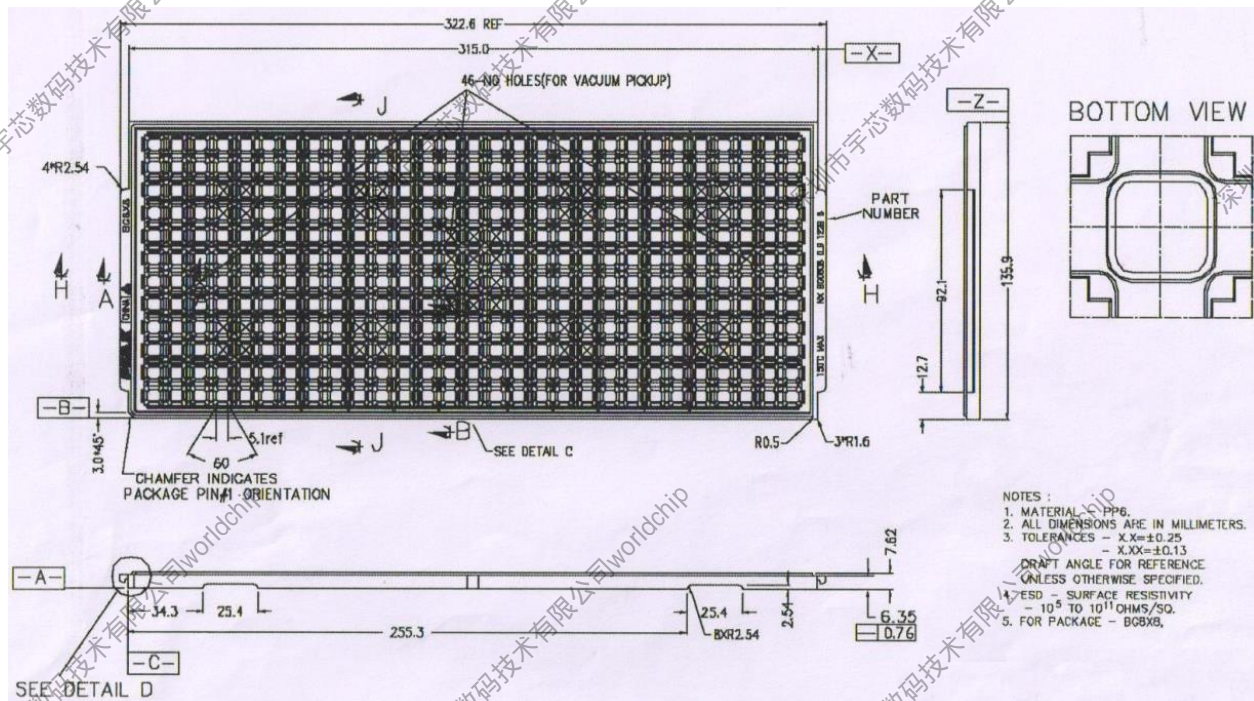
Figure 9-3 Tray Dimension Drawing
