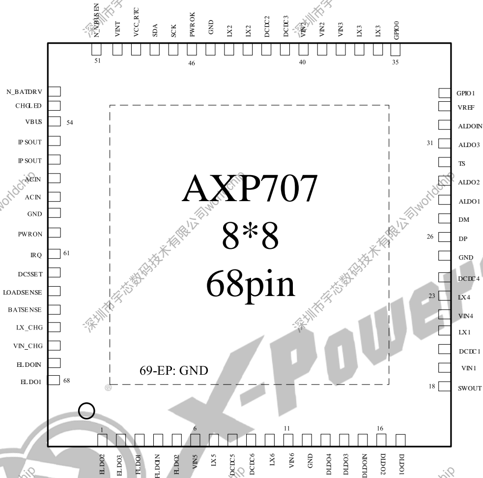
Figure 5-1 Pin Map
