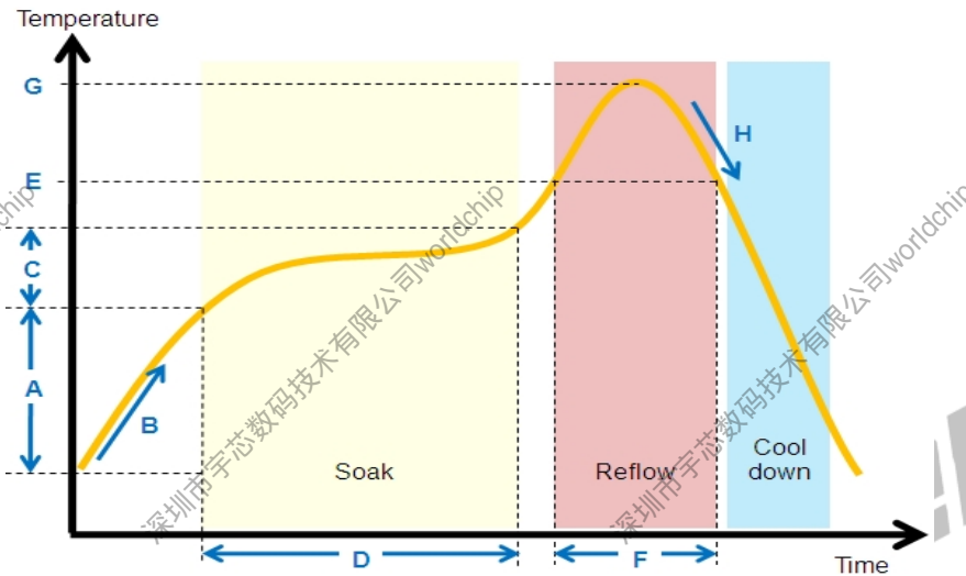
Figure 10-1 AXP707 Typical Reflow Profile
