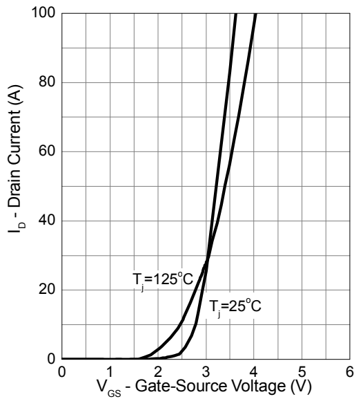
Transfer Characteristics
