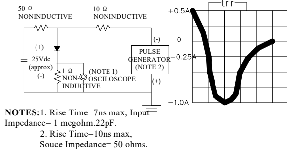
FIG.5-TEST CIRCUIT DIAGRAM AND REVERSE RECOVERY TIME CHARACTERISTIC
