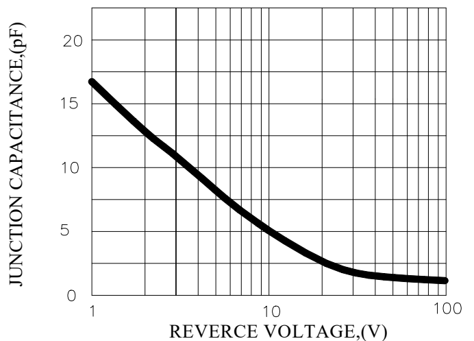
FIG.6-TYPICAL JUNCTION CAPAOTANCE
