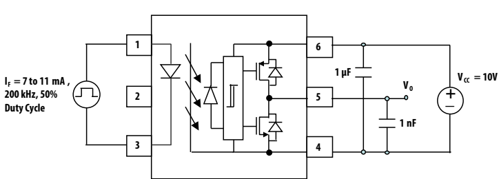
Figure 14: t r and t f Test Circuit and Waveforms
