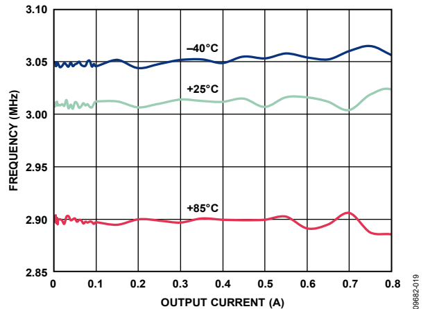
Figure 18. Buck Switching Frequency vs. Output Current, Across Temperature, V_{OUT1} = 1.8\text{ V} , PWM Mode
