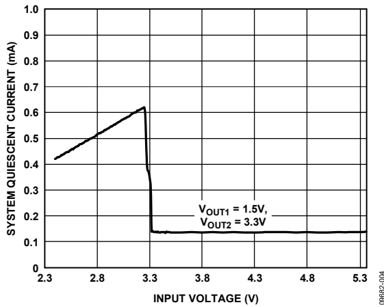
Figure 4. System Quiescent Current (Sum of All the Input Currents) vs. Input Voltage, VOUT1 = 1.5 V, VOUT2 = 3.3 V
