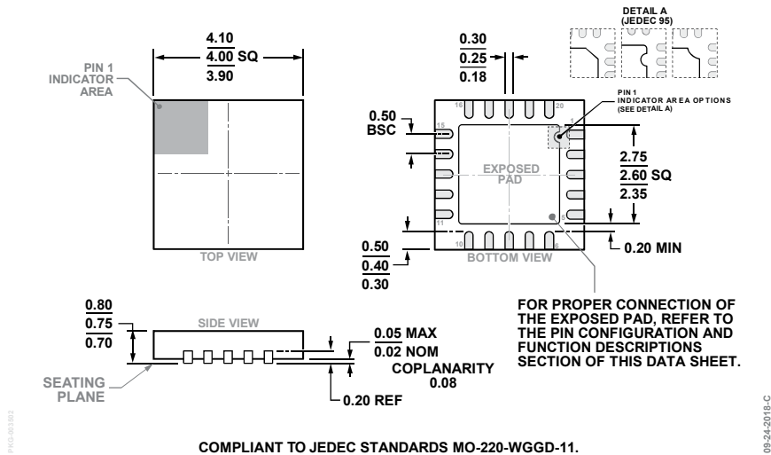
Figure 57. 20-Lead, Lead Frame Chip Scale Package [LFCSP] 4 mm x 4 mm Body and 0.75 mm Package Height (CP-20-8) Dimensions shown in millimeters
