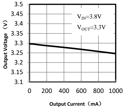
Load Regulation
