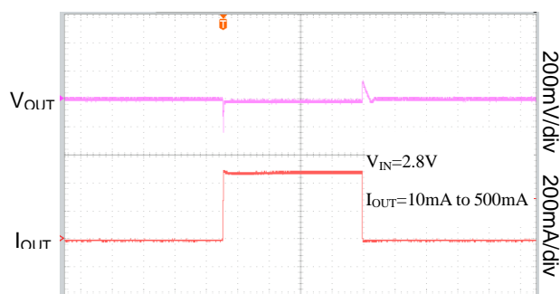
Load Transient Response ( V_{OUT}=1.8V )
