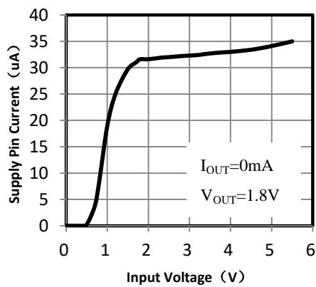
Supply Pin Current vs. Input Voltage
