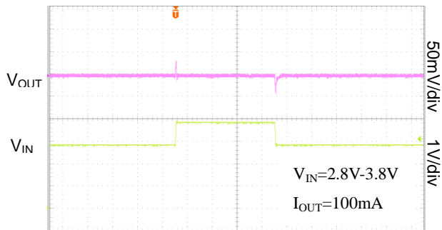
Line Transient Response ( V_{OUT}=1.8V )
