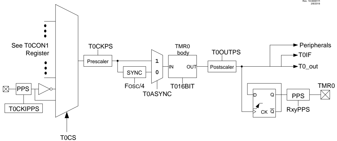
Figure 18-1. Timer0 Block Diagram
