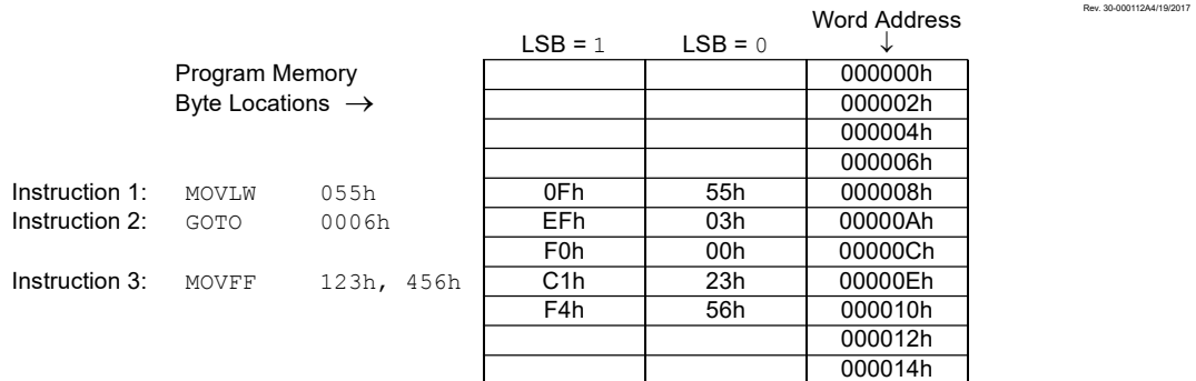
Figure 10-6. Instructions in Program Memory
