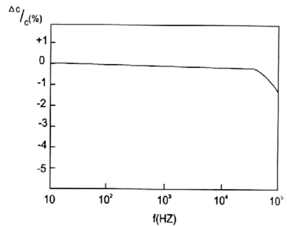
容量变化率与频率的关系 Connections between the capacitance change rate and the frequency
