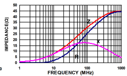
FBC1608-300Y
