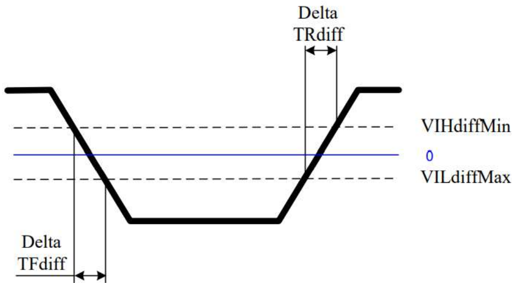
AC and DC Output Measurement Levels
