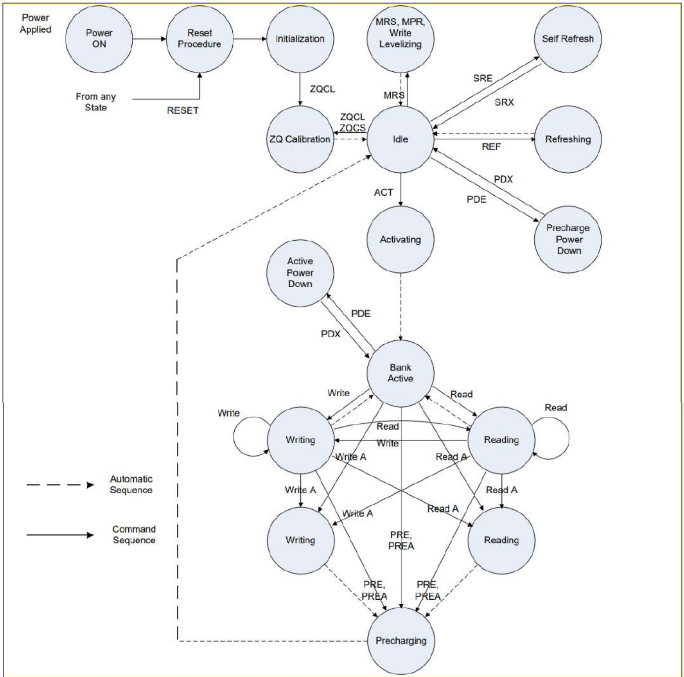
State Diagram Command Definitions
