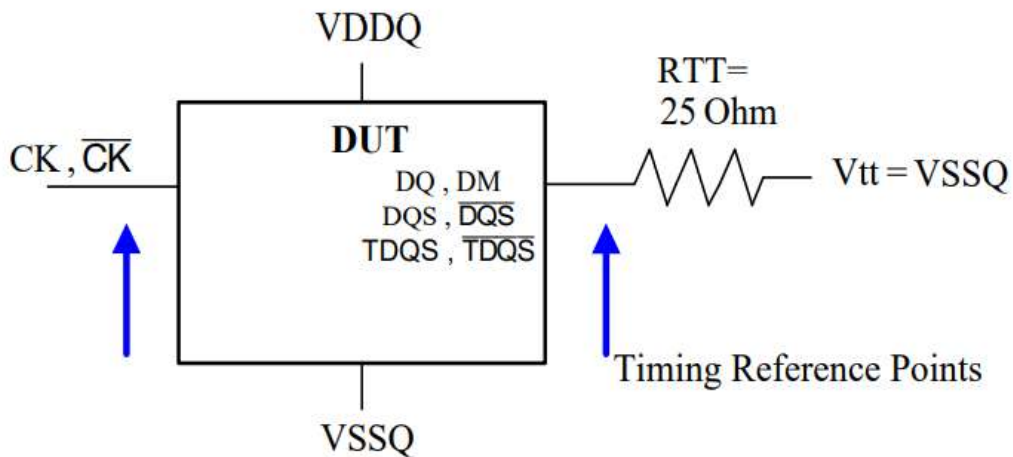
ODT Timing Reference Load
