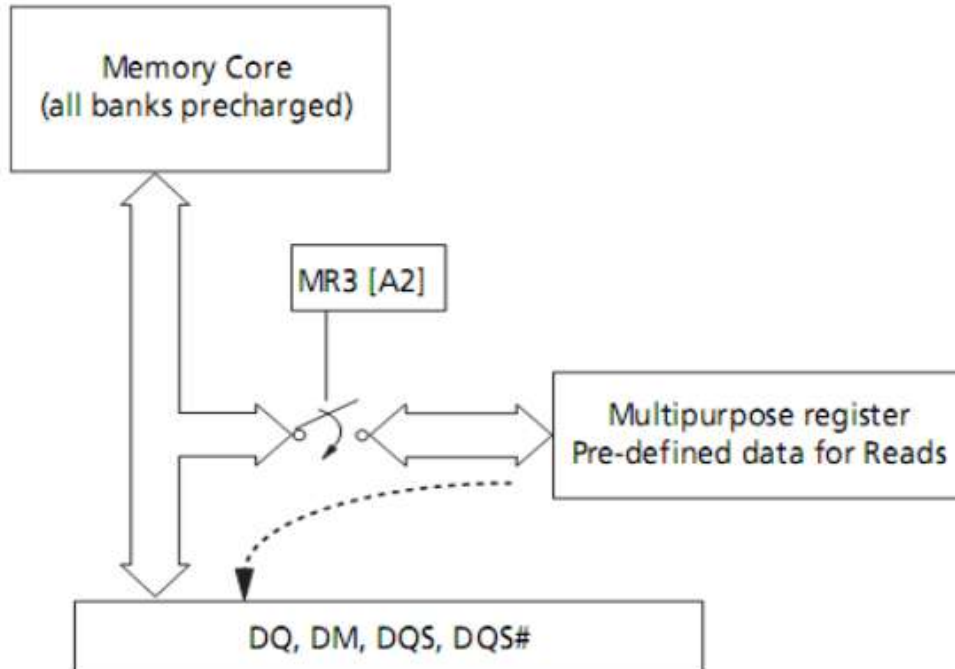
Fig. 1: MPR Block Diagram
