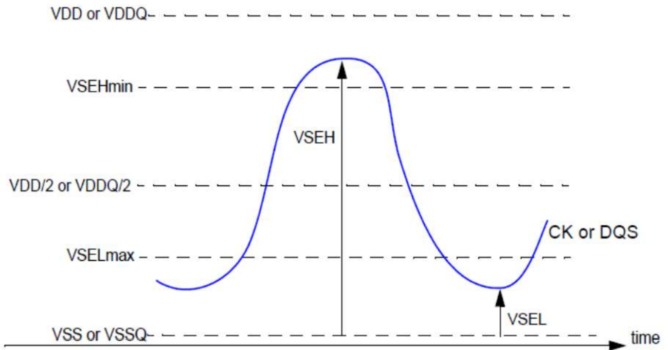
Single-ended requirement for differential signals.
