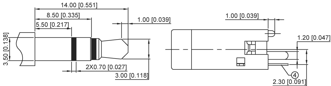
Ø3.50mm 3 POLE PLUG
