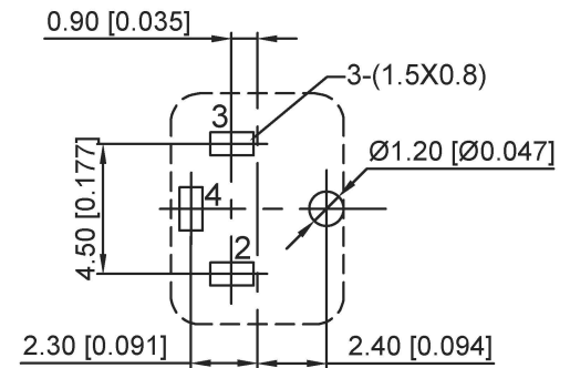
P.C.B LAYOUT MOUNTING PATTERN (TOP VIEW)
