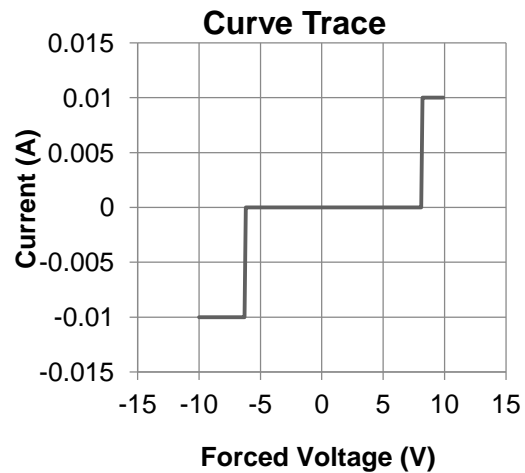
Fig.4 IV Curve
