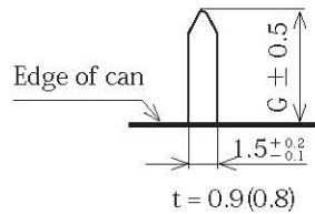
Terminal dimensions
