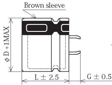
Terminal dimensions
