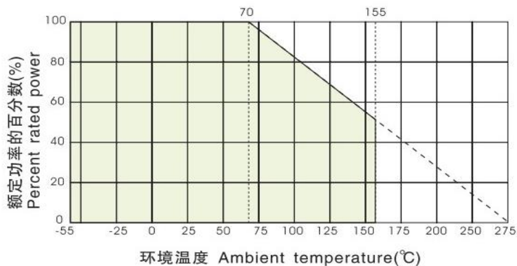
■ 降功耗曲线 Derating Curve
