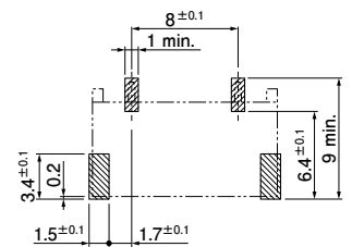
4 mm pitch/ 3-circuit with plugged up hole
