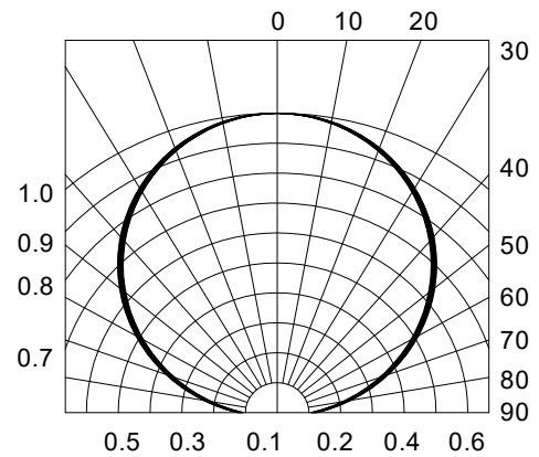
Fig.6-Radiation Diagram Ta=25°C
