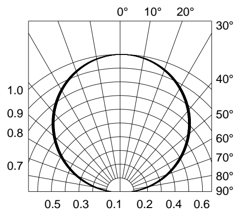
Fig.6-Radiation Diagram Ta=25°C
