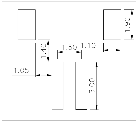
RECOMMENDED P.C.B HOLE LAYOUT
