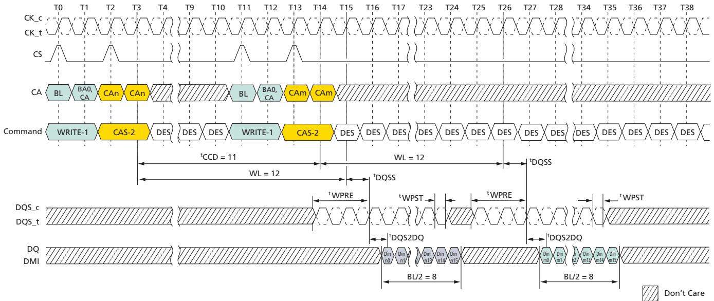
Figure 54: Consecutive Write: t_{CCD} = \text{Min} + 3, 0.5n\text{CK} Postamble
