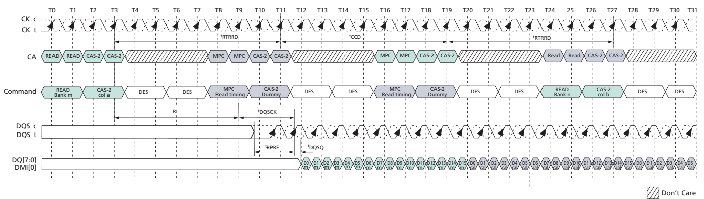
Figure 173: DQ Read Training Timing
