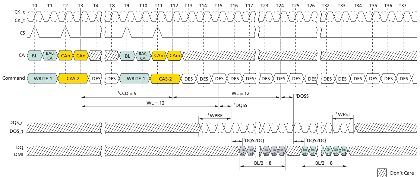
Figure 51: Consecutive Write: t_{CCD} = \text{Min} + 1, 1.5n\text{CK} Postamble
