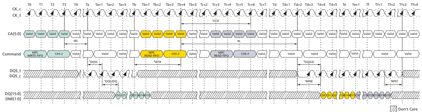
Figure 114: RD-FIFO – t_{WPRE} = 2nCK , t_{WPST} = 0.5nCK , t_{RPRE} = \text{Toggling} , t_{RPST} = 1.5nCK
