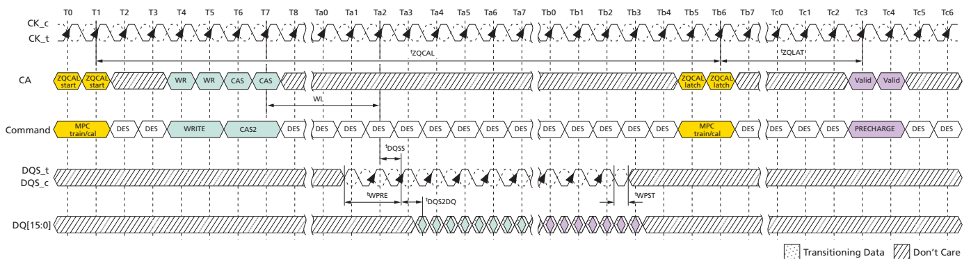
Figure 128: ZQCal Timing
