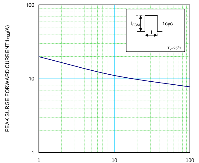
I FSM -t CHARACTERISTICS
