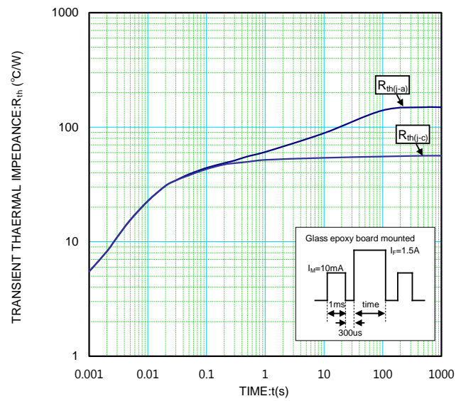
R th -t CHARACTERISTICS
