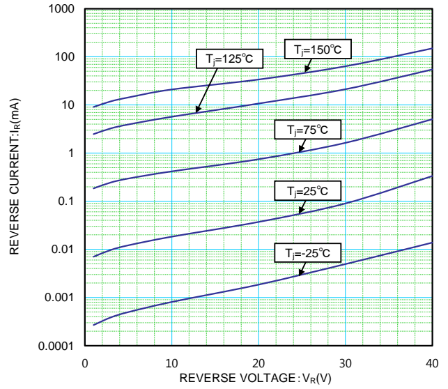
V R -I R CHARACTERISTICS
