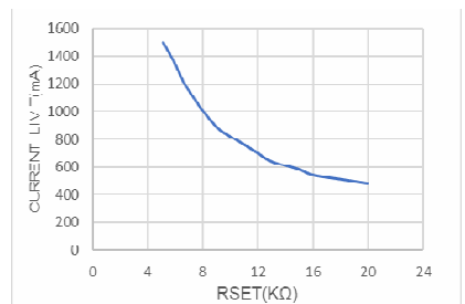
Current Limit vs. R SET I LIM = 0.4~1.5A
