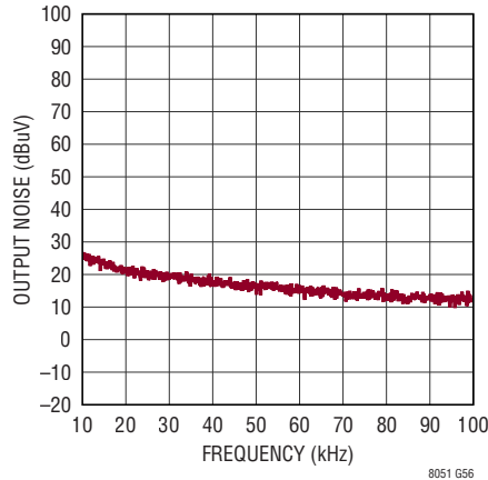
Output Noise Spectrum DC2860A, 100kHz Span V_{IN} = 12\text{V} , V_{OUT} = 3.3\text{V} I_{OUT} = 1.2\text{A} , f_{SW} = 1.2\text{MHz}
