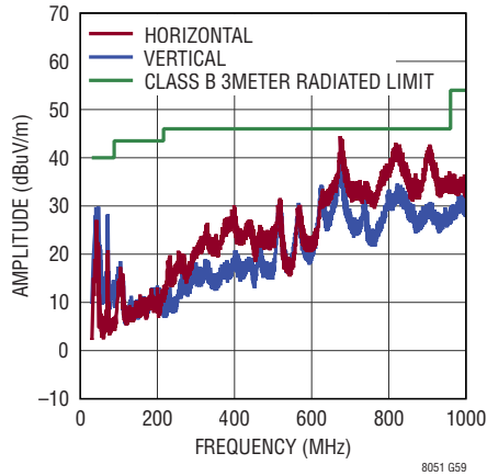
CISPR22 Class B Emissions DC2860A Demo Board V_{INn} = 12\text{V} , I_{OUTn} = 1.2\text{A} 5V_{OUT1} , 3.3V_{OUT2} , 2.5V_{OUT3} , 1.8V_{OUT4} Spread Spectrum On, No EMI Filter
