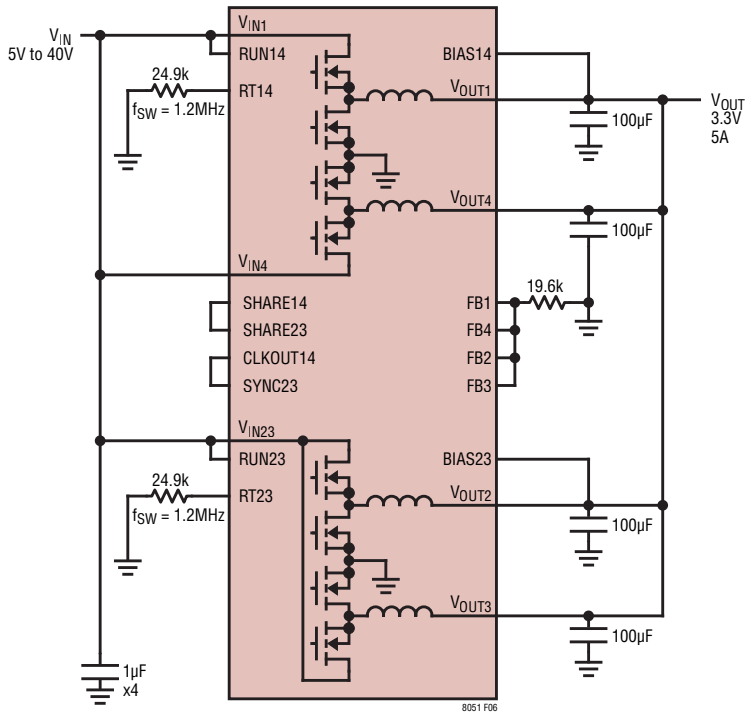
PINS NOT USED: TRSS1, TRSS2, TRSS3, TRSS4, PG1, PG2, PG3, PG4, SYNC14, CLKOUT23, VCC14, VCC23
