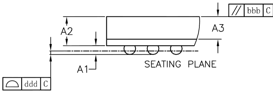
DETAIL A(2:1)
