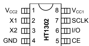
SO (208mils/150mils)
