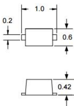
Dimensions (mm)
