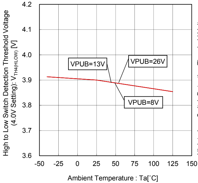
Figure 77. High to Low Switch Detection Threshold Voltage (4.0V Setting) vs Ambient Temperature
