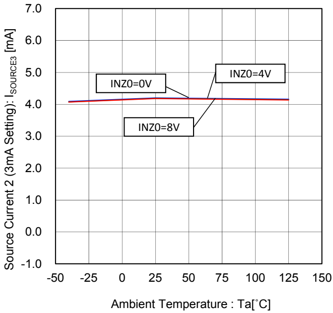
Figure 41. Source Current 2 (3mA Setting) vs Ambient Temperature
