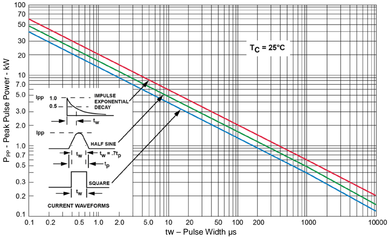
FIGURE 1 Peak Pulse Power vs Pulse Time
