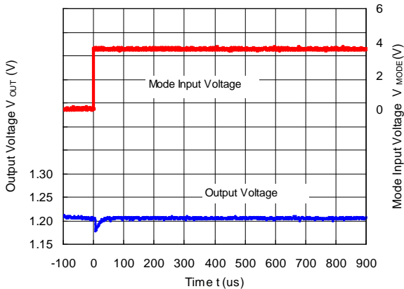
RP506Kxx1A/B/C (V_{IN} = 3.6\text{ V} , V_{OUT} = 1.2\text{ V} , I_{OUT} = 1\text{ mA} ) MODE = "L" --> MODE = "H"
