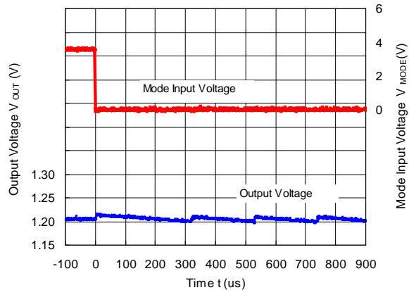
RP506Kxx1A/B/C (V_{IN} = 3.6\text{ V} , V_{OUT} = 1.2\text{ V} , I_{OUT} = 1\text{ mA} ) MODE = "H" --> MODE = "L"
