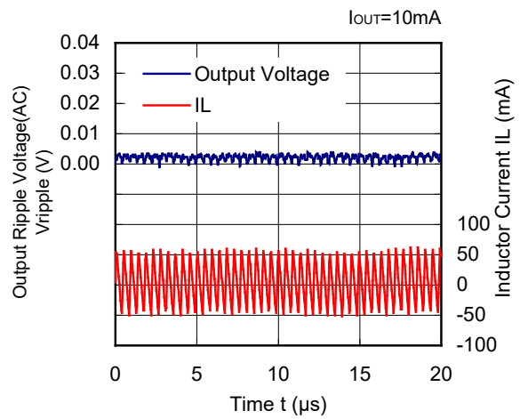
RP505K V_{OUT}=1.2V(V_{IN}=3.6V) MODE="H" forced PWM
