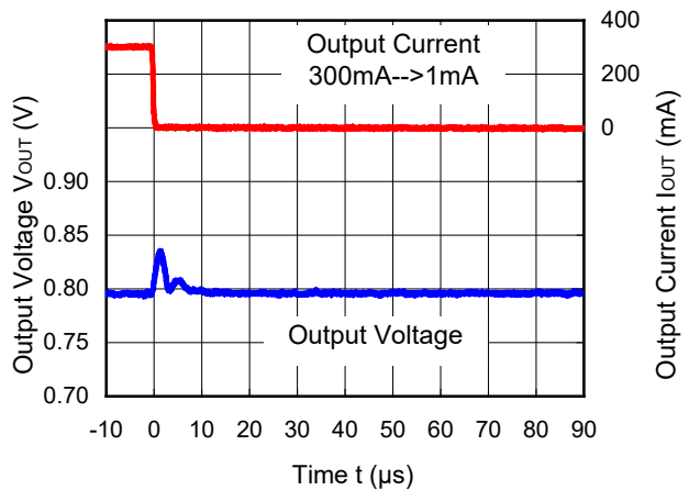
RP505K081A/B ( V_{IN}=3.6V ) MODE="H" forced PWM
