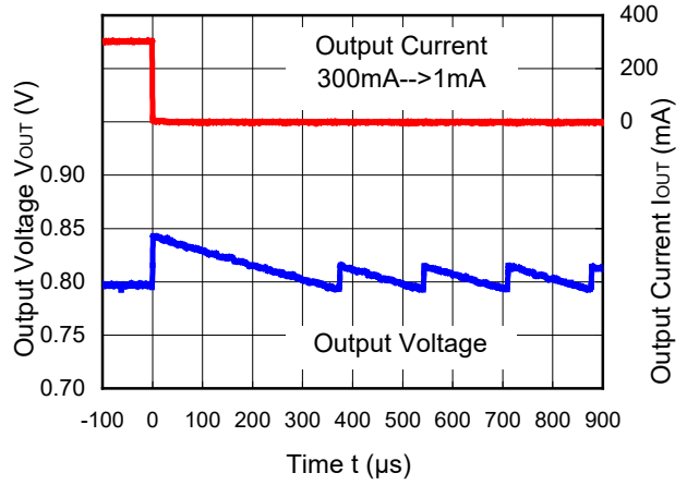
RP505K081A/B ( V_{IN}=3.6V ) MODE="L" PWM/VFM automatic shift
