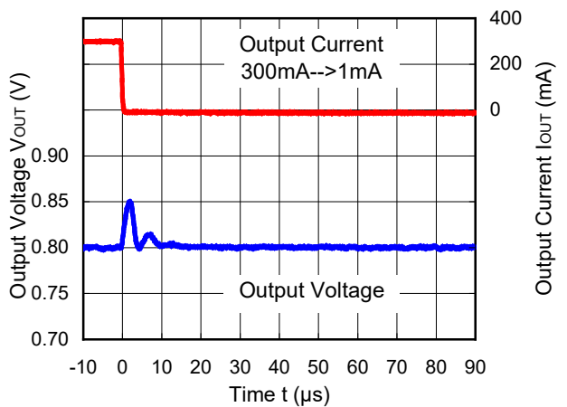
RP505K001C ( V_{IN}=3.6V , V_{OUT}=0.8V ) MODE="H" forced PWM
