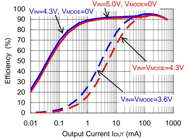
RP504x V_{OUT} = 3.3\text{ V}
