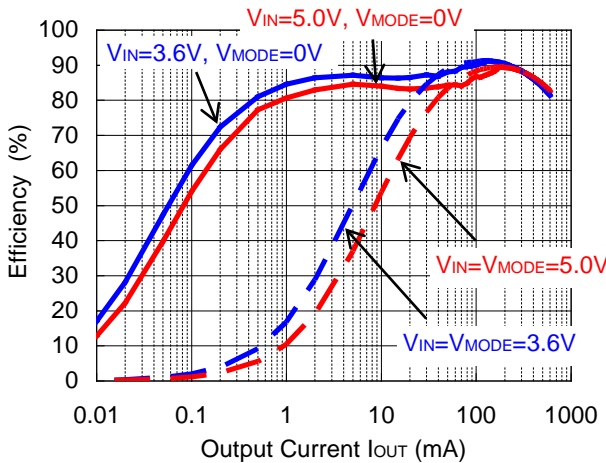
RP504x V_{OUT} = 1.8\text{ V}
