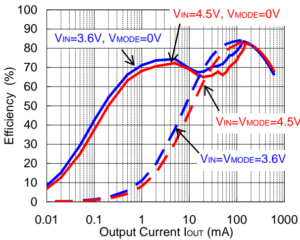
RP504x V_{OUT} = 0.8\text{ V}
