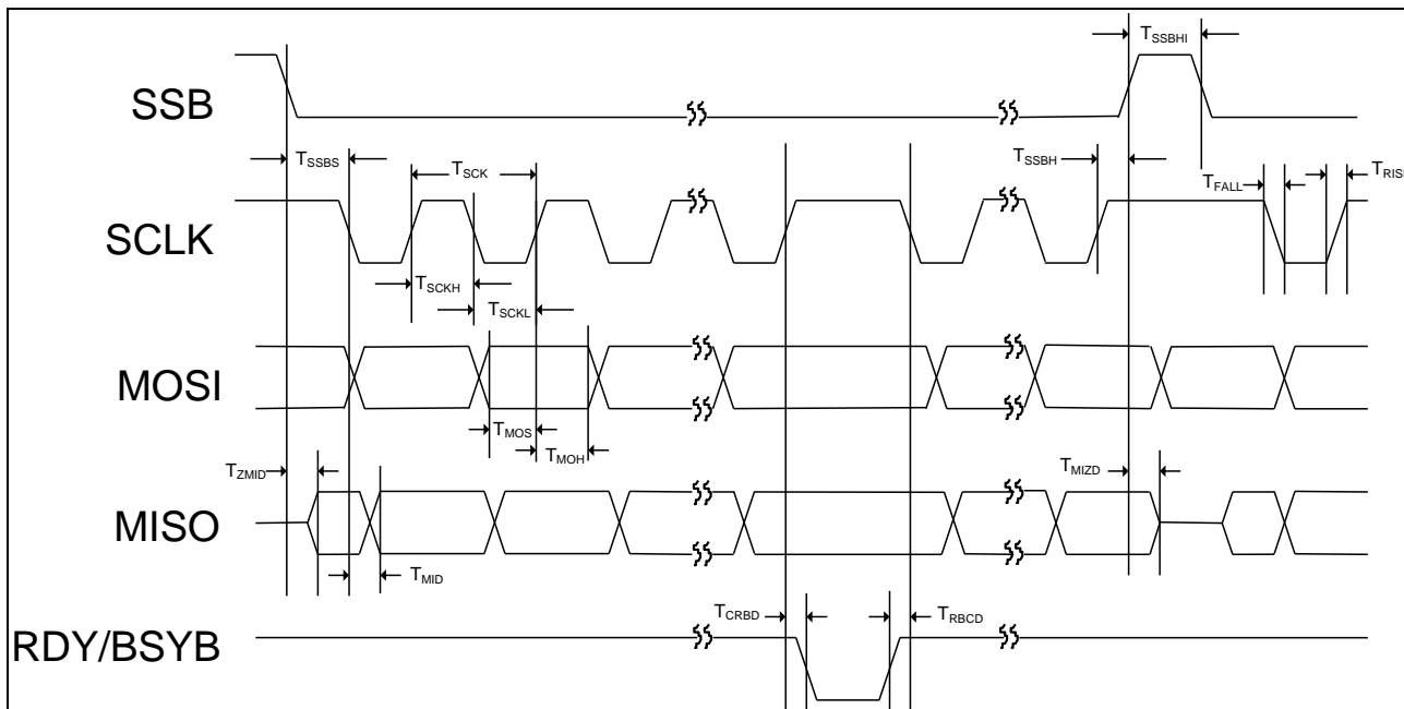
Figure 12-1 SPI Timing
