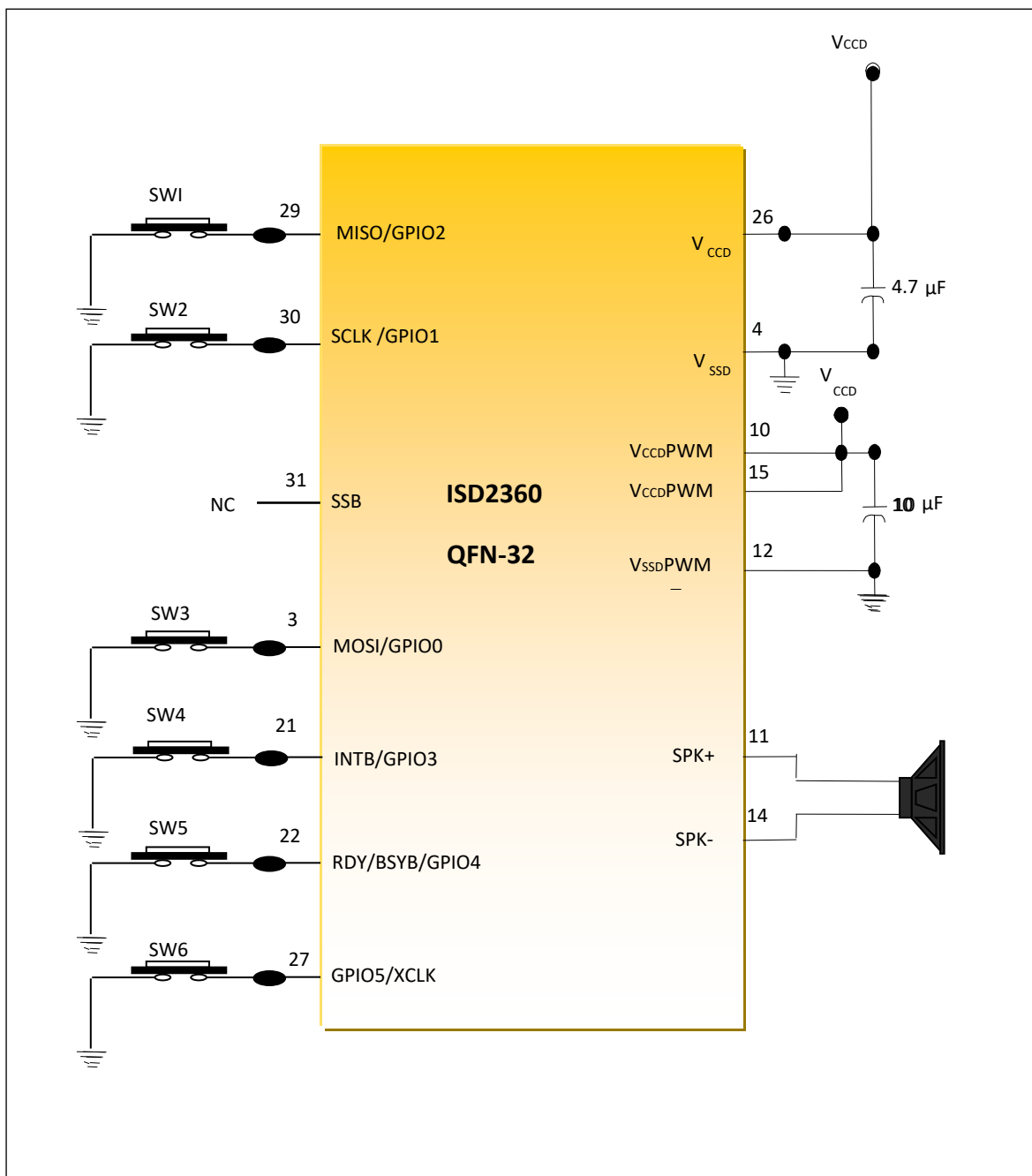
Figure 135-2 ISD2360 Application Diagram Stand-Alone Mode
