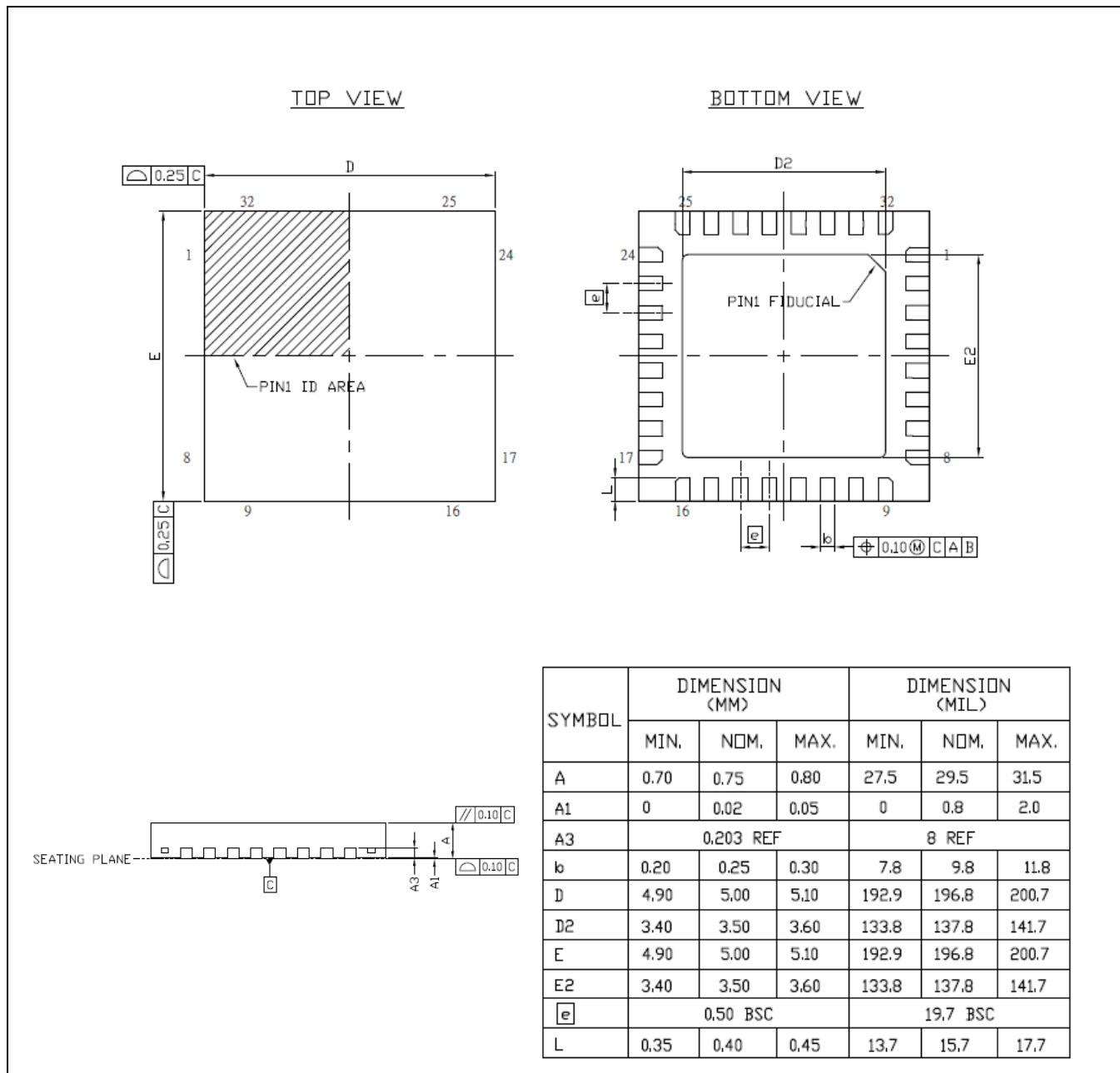
Figure 14-1 QFN 32 - Lead Package QFN 32L 5X5 mm 2 , Thickness 0.8 mm(Max) , Pitch 0.5 mm (Saw Type) TICP EP SIZE 3.5X3.5 mm 2
