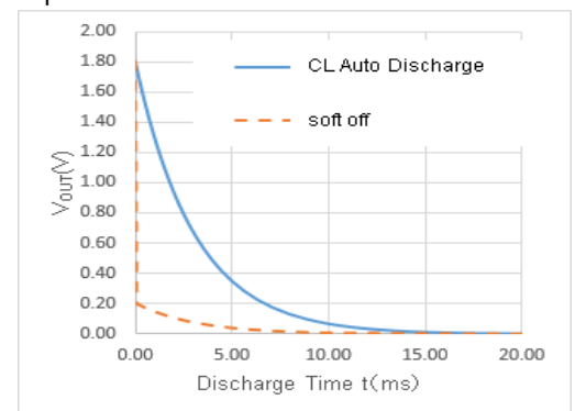
Soft-off function vs C L High Speed Discharge C L = 47μF
