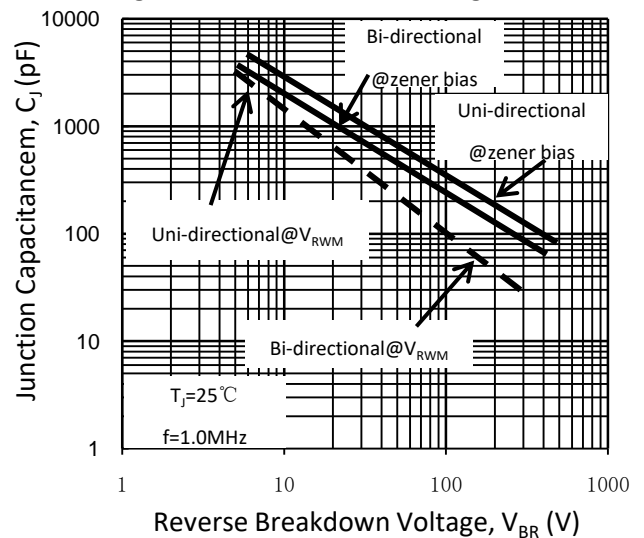
Fig. 6-Typical Junction Capacitance
