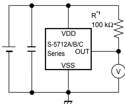
Figure 8 Test Circuit 4
