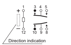
Schematic (Bottom view) Single side stable
