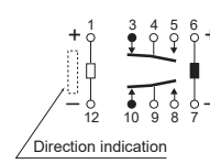
Schematic 2 coil latching (Bottom view)
