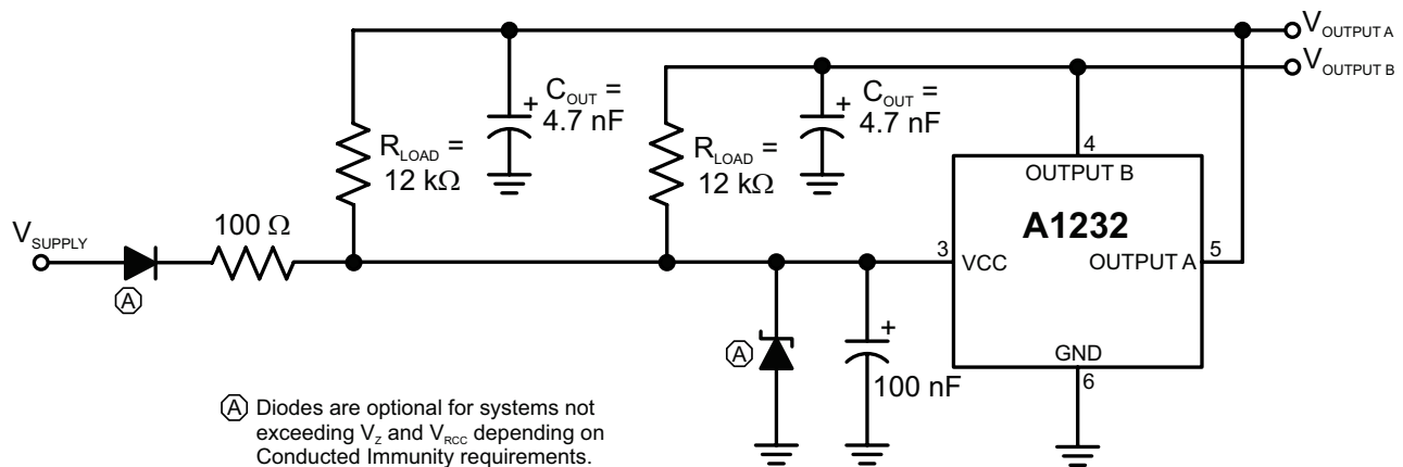
Figure 11: Typical Application Circuit for Unregulated Power Supply
