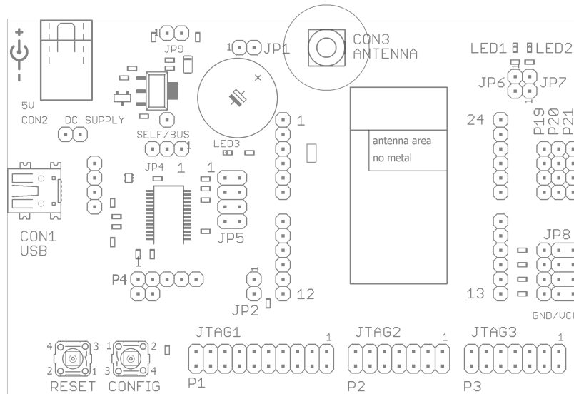
Figure 13: Assembly diagram
