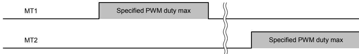
Figure 7.21 PWM Drive
