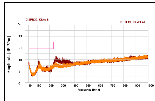
FIGURE 1: Radiated Emissions, CISPR32, Class B ( V_{IN} = 5V , V_{OUT} = 1V , I_{OUT} = 6A ).
