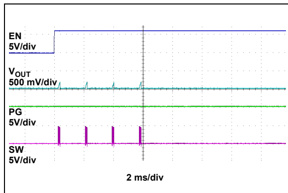
FIGURE 2-23: Power-up into Short Circuit.
