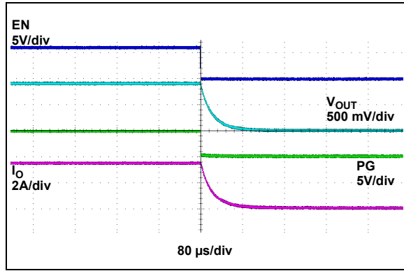
FIGURE 2-21: EN Turn-Off, R_{LOAD} = 0.3\Omega .
