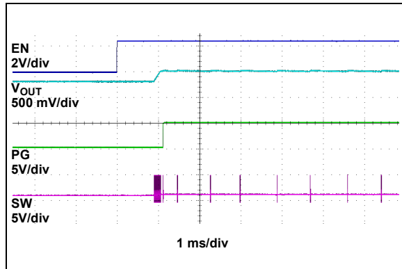
FIGURE 2-22: EN Turn-On into Pre-Biased Output ( V_{pre-bias} = 0.8V ).
