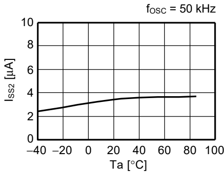
(3) Current Consumption at Shutdown ( I_{\text{SSS}} ) vs. Temperature ( T_a )
