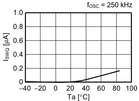
(5) Switching Transistor Leakage Current ( I_{\text{swQ}} ) vs. Temperature ( T_a )
